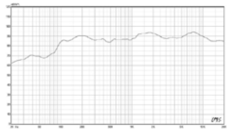
Frequency Response Graph:
