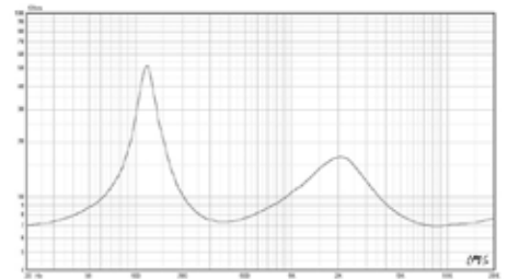
Impedance Graph:
